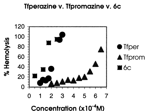
Figure 2. The percentage of hemolysis induced by T.f.prom. ( \blacktriangle ), T.f.per. ( \bullet ), and 6c ( \blacksquare ). The percentage of hemolysis was determined against a sample of red blood cells lysed with distilled water. Each of the curves was derived from at least three runs, and demonstrated significant consistency.
